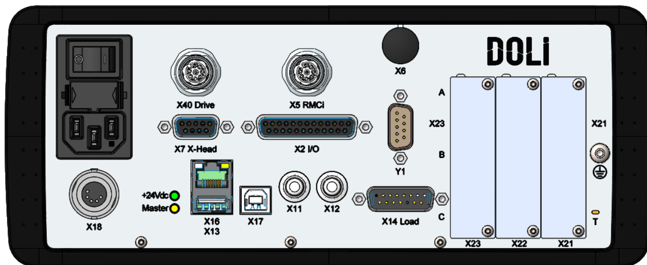
Fig. 12: Rear view EDCi22/52 with external X40 DriveBox
